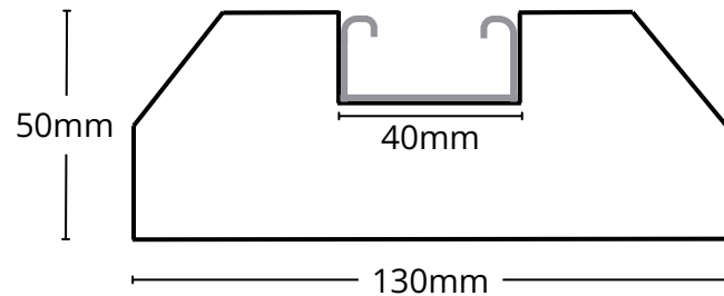
CROSS SECTION - ACM250 & ACM400
